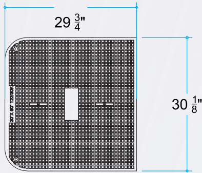
COVER TOP VIEW
