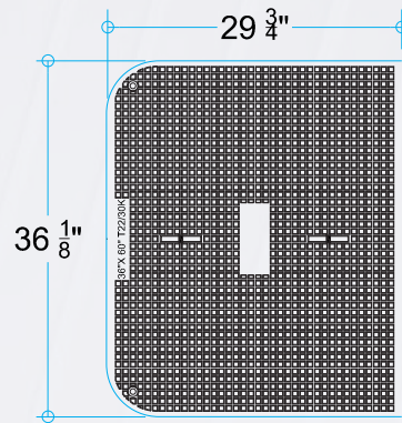
COVER TOP VIEW
