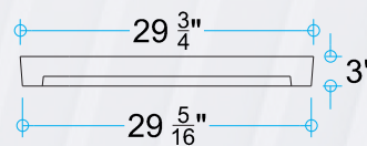
COVER FRONT VIEW
